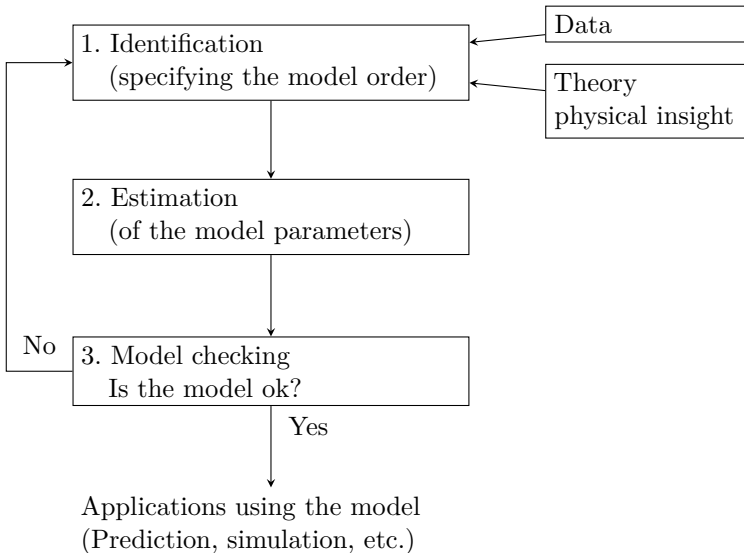
Figure 6.1: Principles for model building.
