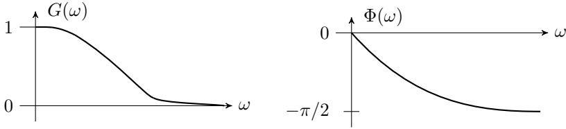
Figure 4.1: Amplitude (gain) and phase for an RC -element.
