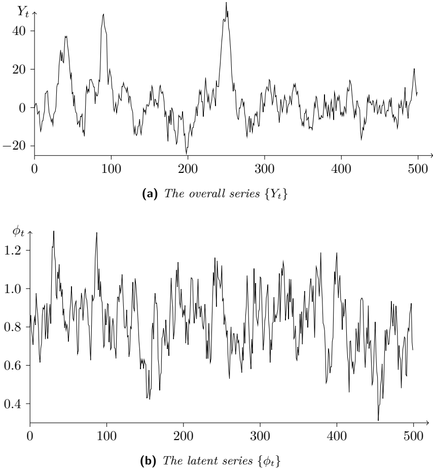
Figure 11.3: (a) The overall series \{Y_t\} and (b) the latent series \{\phi_t\} .
